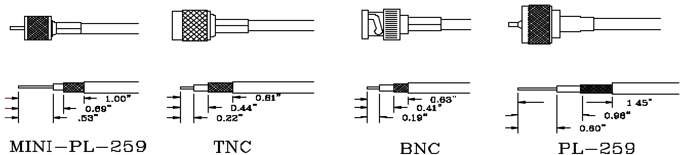
Cable Stripping Dimensions
