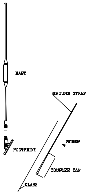
Figure 5 – General Assembly
