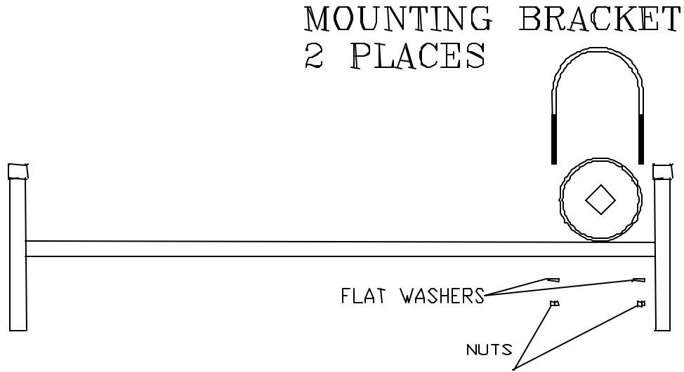
Figure 3 – Mounting Procedure
