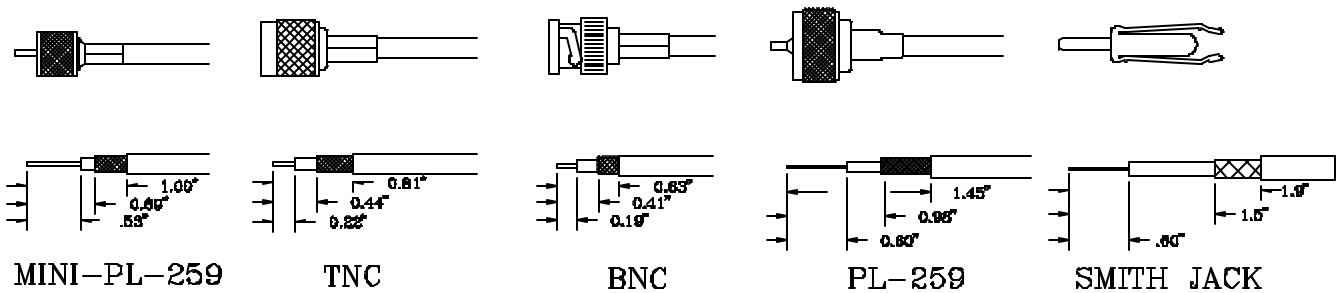
Cable Stripping Dimensions
