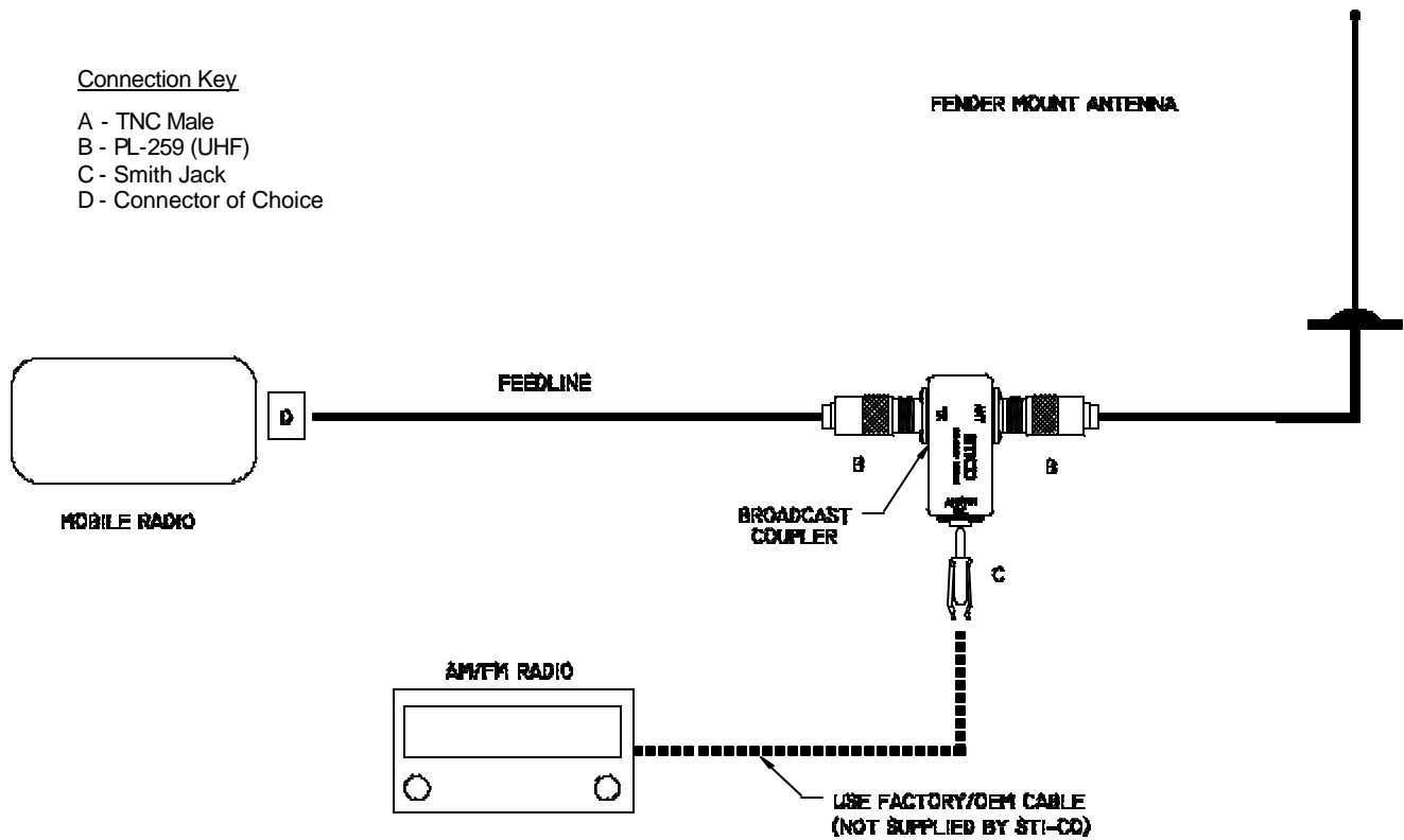
VHF Fender Mount Antennas
