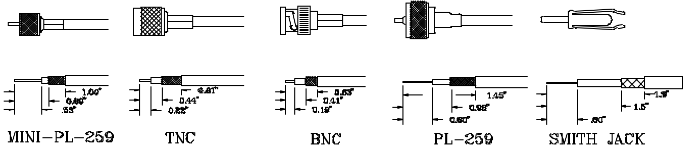
Cable Stripping Diagram
