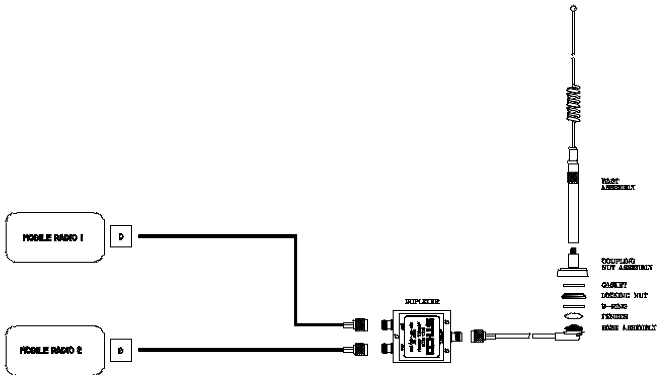
UHF/Cellular Dual Band Antenna Installation Diagram
